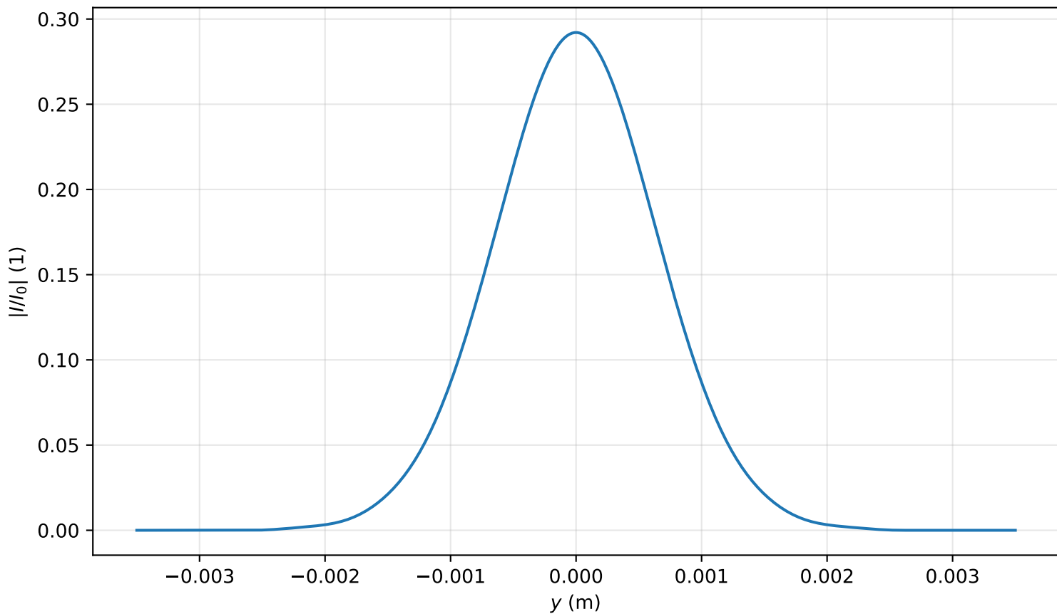
Intensity profile I(x=0, y, z=3.582)/I_0 , P_{in}=0.2P_{cr} , artificial time
